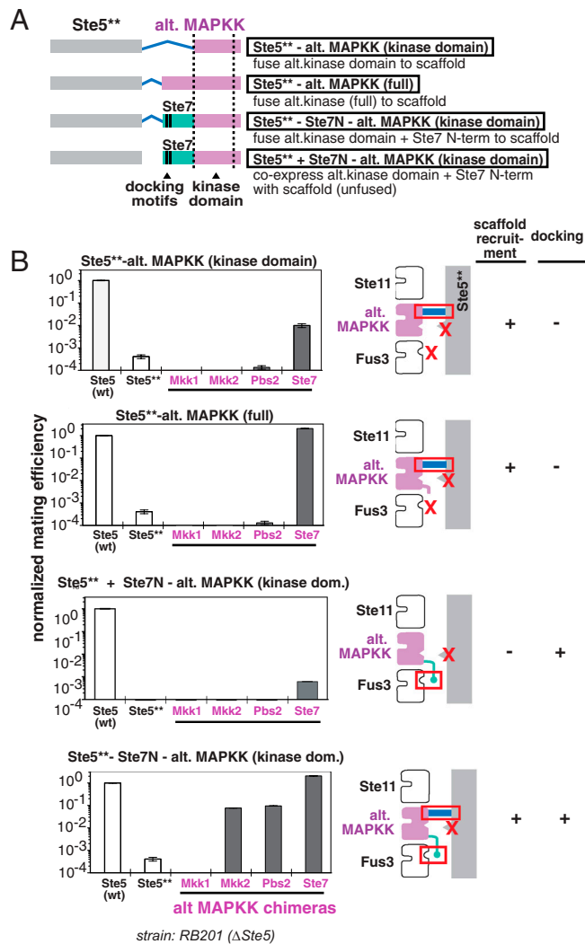
Fig. 3. Alternative MAPKKs can functionally replace Ste7 if proper scaffold tethering and docking interactions are added. (A) Constructs used to test Ste7 functional replacement using alternative yeast MAPKKs. The green box represents a.a. 1–190 of Ste7, containing the docking motifs for Fus3. Although omitted for simplicity, each construct is HA-tagged (C terminus) and expressed from the Ste5 promoter. (B) Quantitative mating assays with alternative MAPKK constructs. Mating efficiencies were normalized to that of Ste5 (wild-type). Background mating efficiency is \leq 10^{-4} . The blue bar in the schematic represents the covalent fusion to Ste5. The green arm represents a.a. 1–190 of Ste7. The magenta arm represents the endogenous N terminus of each alternative MAPKK. Chimeric constructs were expressed from the Ste5 promoter on pRS316 derived plasmids, in a \Delta ste5 strain (RB201). In the case of the Ste5** + Ste7N-altMAPKK (kinase domain) pairs of constructs, Ste5** was expressed from the Ste5 promoter on pRS316 derived plasmids, while the Ste7N-altMAPKK kinase domain was expressed from the Adh1 promoter on pRS314 derived plasmids. Data are average of three repeats.
