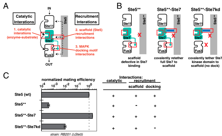
Fig. 2. Both catalytic and recruitment interactions are necessary for MAPKK Ste7 function. (A) Schematic of the kinase cascade of the pheromone response pathway. Red boxes indicate the methods utilized by Ste7 for network connectivity: active site recognition, docking interactions, and interactions with the Ste5 scaffold. (B) Strategy for testing contribution of scaffolding and docking interactions to Ste7 function. Mating assays were performed with a Ste5 scaffold with selective mutations V763A/S861P that destroys native Ste7 binding to Ste5 (Ste5**) (19) (depicted by red X). Ste7 was either untethered to Ste5, tethered to Ste5 by being expressed as a fusion to the Ste5 C terminus (indicated by blue bar), or tethered to Ste5 but with its Fus3 docking sites (green arm) deleted. (C) Quantitative mating assays with Ste7 recruitment mutants. Mating efficiencies were normalized to that of Ste5 (wild-type). Background mating efficiency is \leq 10^{-4} . Chimeric kinases were expressed from the Fus3 promoter on a pRS516 derived plasmid, in a \Delta Ste5 strain (RB201). Data are average of three repeats.
