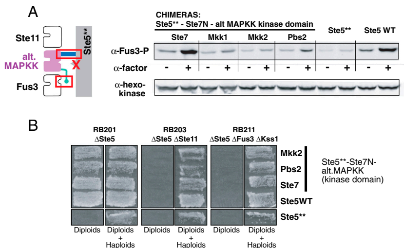
Fig. 4. Alternative MAPKK chimeras that able to functionally replace Ste7 signal through the proper upstream and downstream partners. (A) The alternative MAPKK chimeras that functionally replace Ste7 show alpha-factor induced phosphorylation of the mating MAPK Fus3. Western blots are shown for samples after 10 min of alpha-factor stimulation, probed with the anti-p42/44 antibody (cell signaling #4370). Here MAPKK chimeras are expressed from the Ste5 promoter. (B) Complementation of mating deficiency in ste5 \Delta , ste5 \Delta ste11 \Delta , or ste5 \Delta fus3 \Delta kss1 \Delta cells when Ste7 is replaced by alternative MAPKKs that contain both Ste5 scaffold recruitment and Ste7 docking interactions. Growth on diploid selective media indicates cells are capable of mating. Here, the absence of growth indicates that the alternative kinases require both Ste11 and Fus3/Kss1 for a mating phenotype. Chimeric kinases were expressed from Ste5 promoter on pRS316 derived plasmids.
