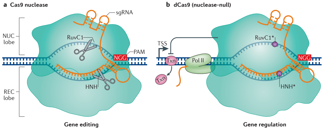
Figure 1 | Gene editing versus gene regulation using Streptococcus pyogenes Cas9 and dCas9. a | The S. pyogenes Cas9 endonuclease consists of a nuclease (NUC) lobe and a recognition (REC) lobe. Cas9 is targeted to specific DNA sequences by direct pairing of the chimeric single guide RNA (sgRNA) with the target DNA. This targeting relies on the presence of a 5' protospacer-adjacent motif (PAM) in the DNA, which in S. pyogenes is usually NGG. Binding mediates cleavage of the target sequence by two nuclease domains, RuvC1 and HNH. b | The S. pyogenes dCas9 protein contains mutations in its RuvC1 (D10A) and HNH (H841A) domains, which inactivate its nuclease function (circles). dCas9 retains the ability to target specific sequences through the sgRNA and PAM. dCas9 binding downstream of the transcription start site (TSS) can block transcription elongation by blocking RNA polymerase II (Pol II) or the binding of important transcription factors (Txn).
